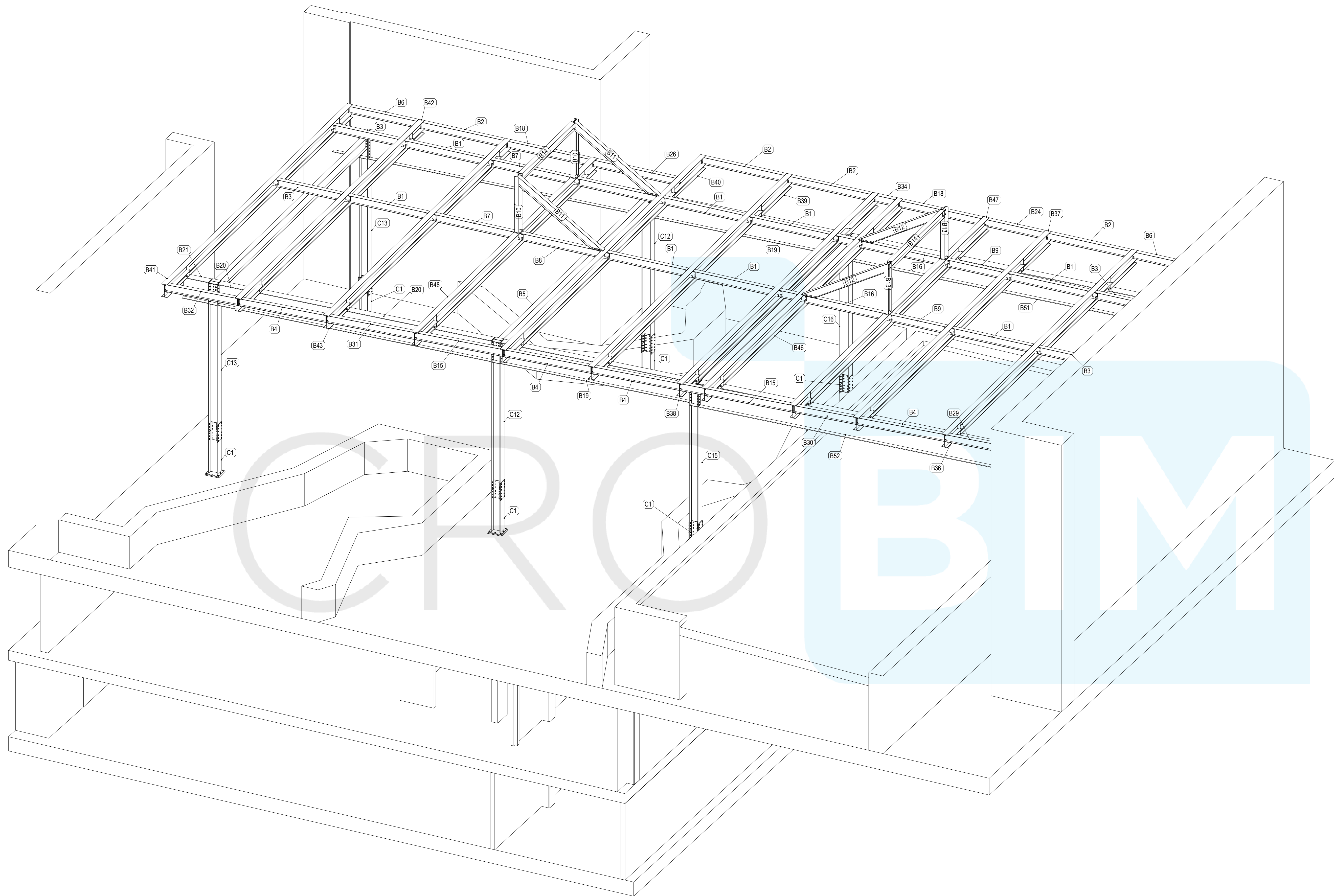
LINK BRIDGE 3D VIEW Scale: 1:60
