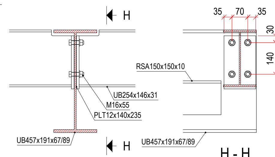
UB457x191x67/89 to UB254x146x31 (EDGE) Scale: 1:10
