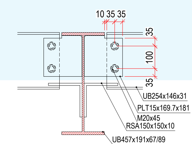
UB457x191x67/89 to UB254x146x31 Scale: 1:10
