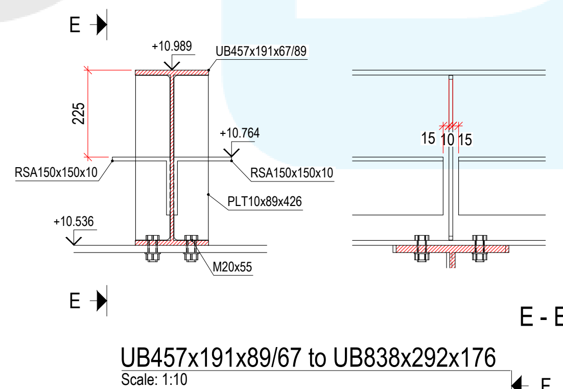
MAIN FRAME CONNECTIONS Scale: 1:10
