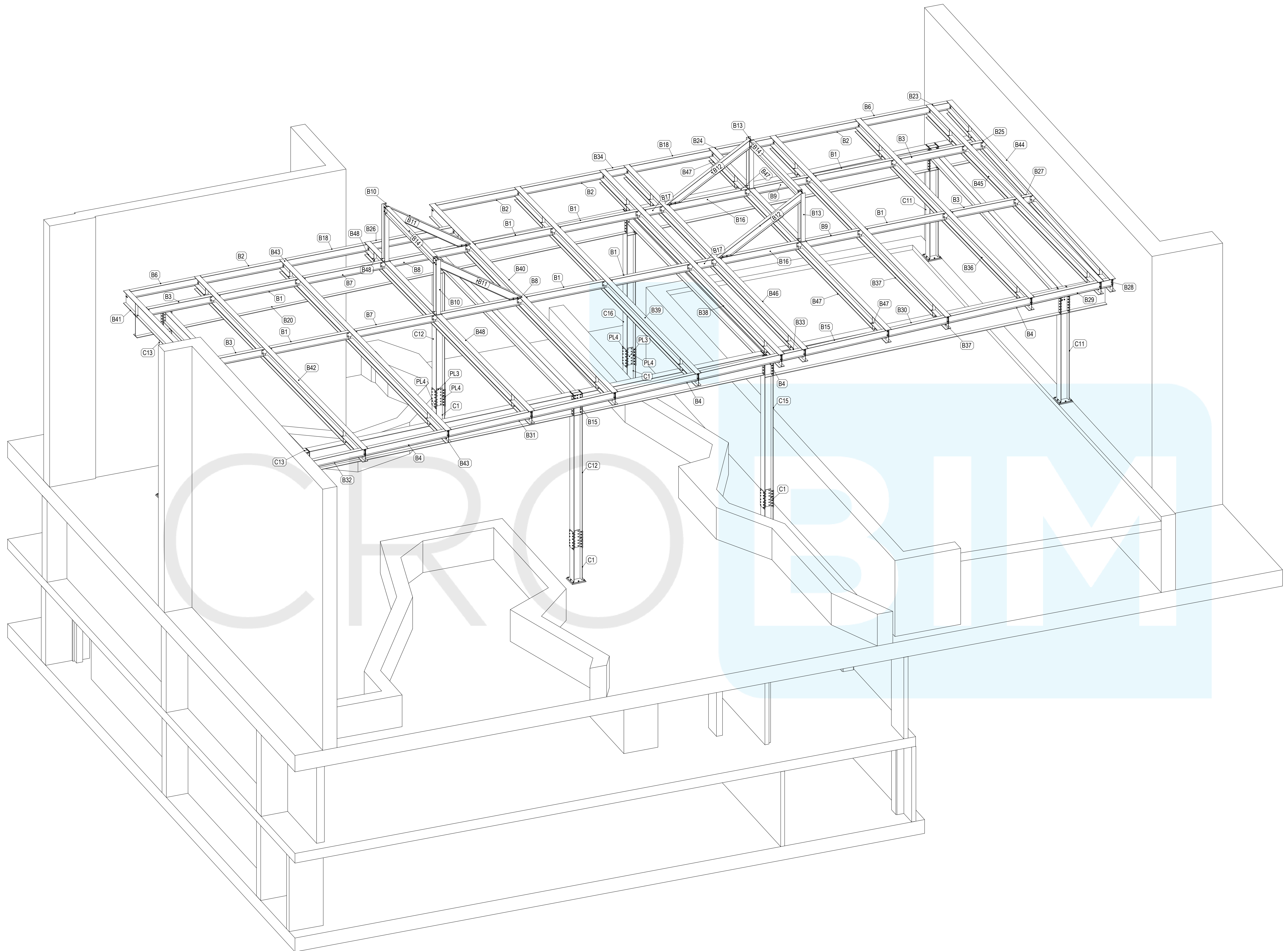
LINK BRIDGE 3D VIEW Scale: 1:60
