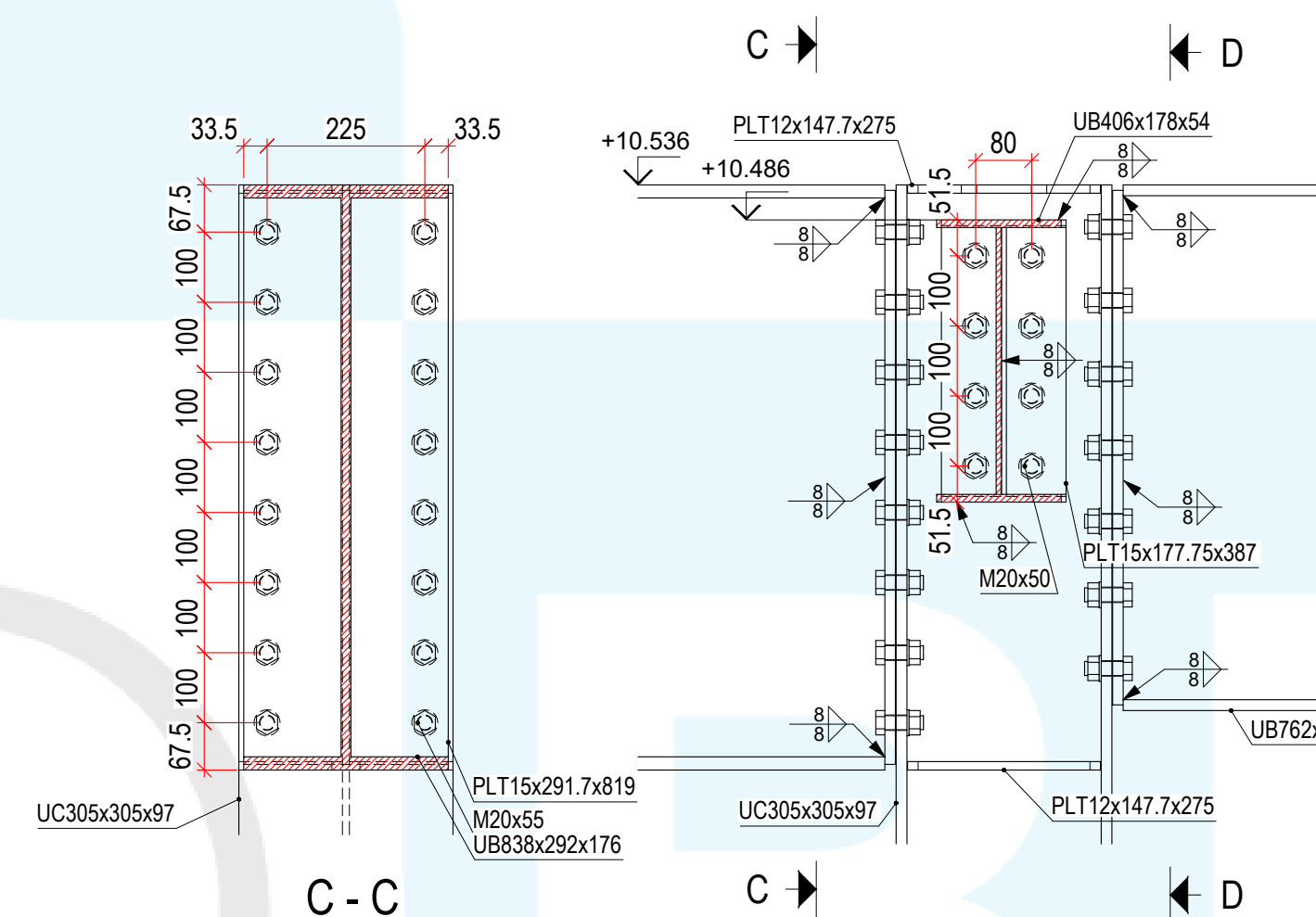
MAIN FRAME CONNECTIONS Scale: 1:10
