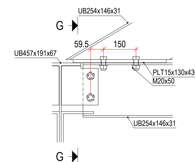
UB254x146x31 to MAIN FRAME Scale: 1:10
