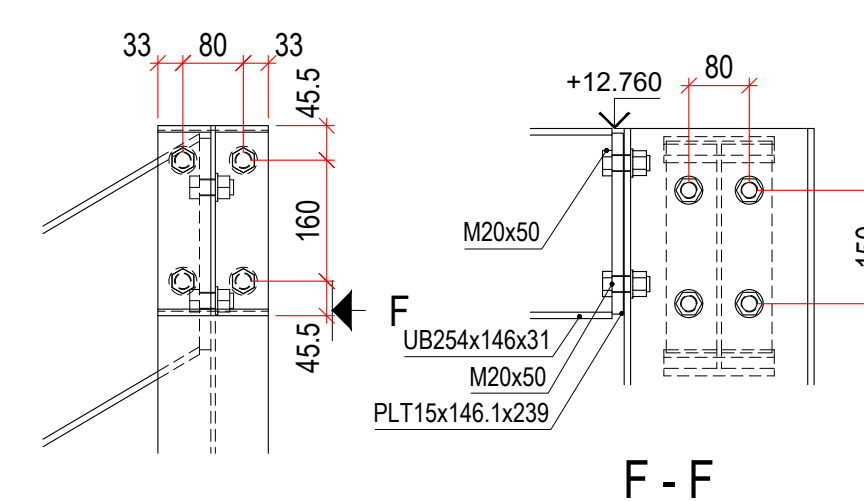
UB254x146x31 to UB254x146x31 Scale: 1:10
