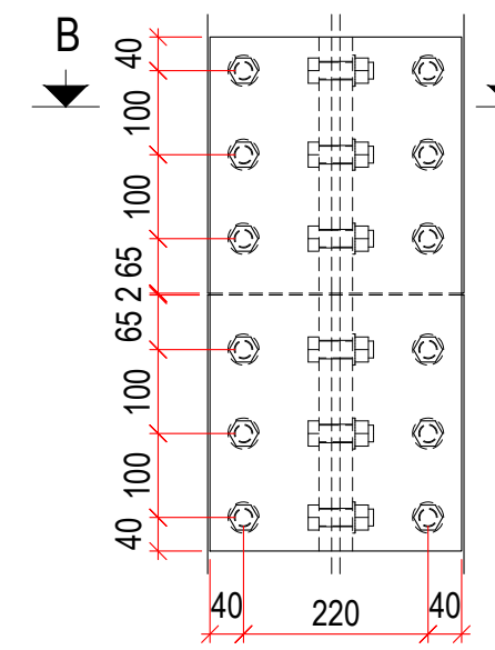
UC305x305x97 SPLICE CONNECTION
