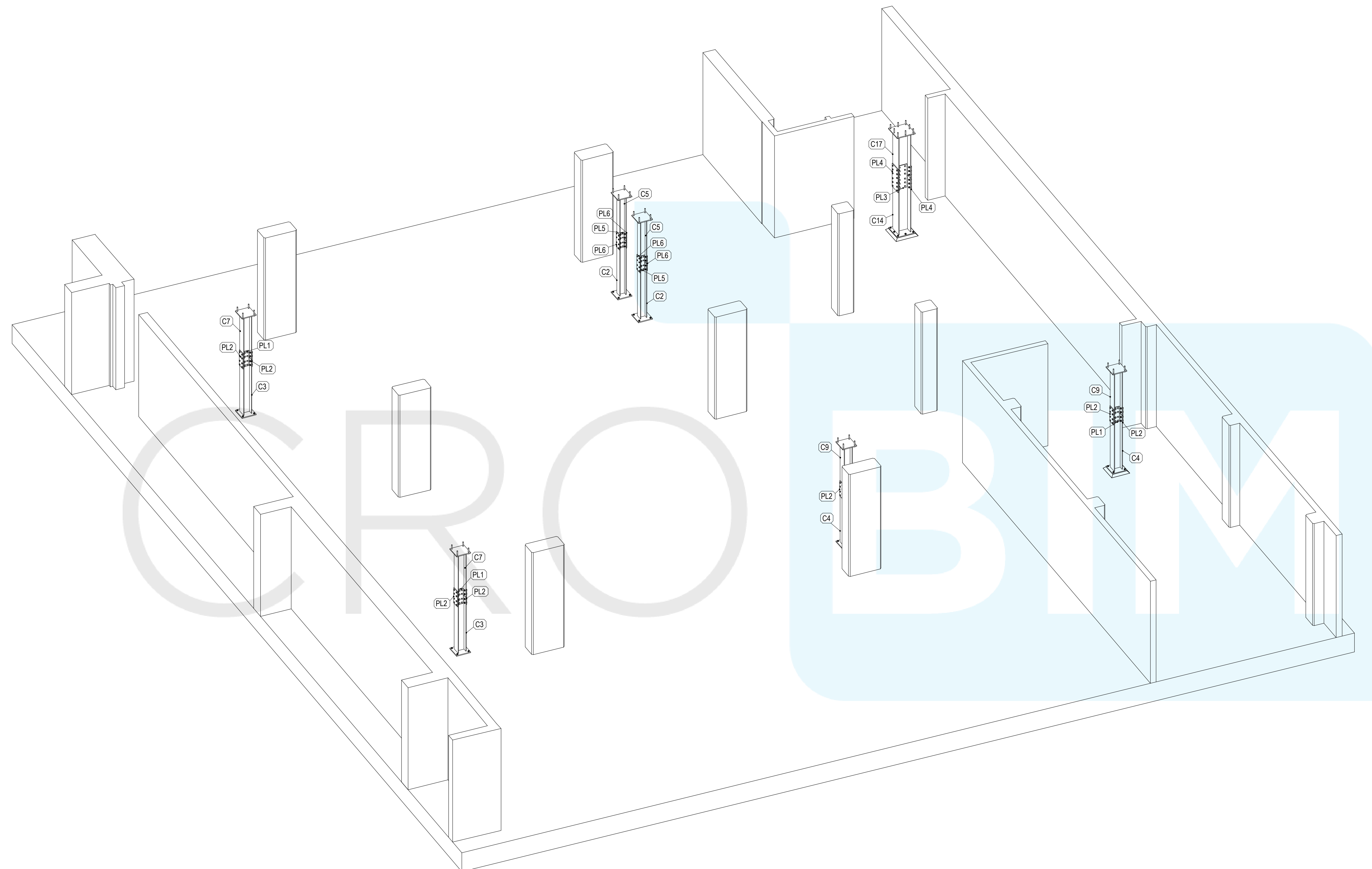
LEVEL B2 3D VIEW Scale: 1:50
