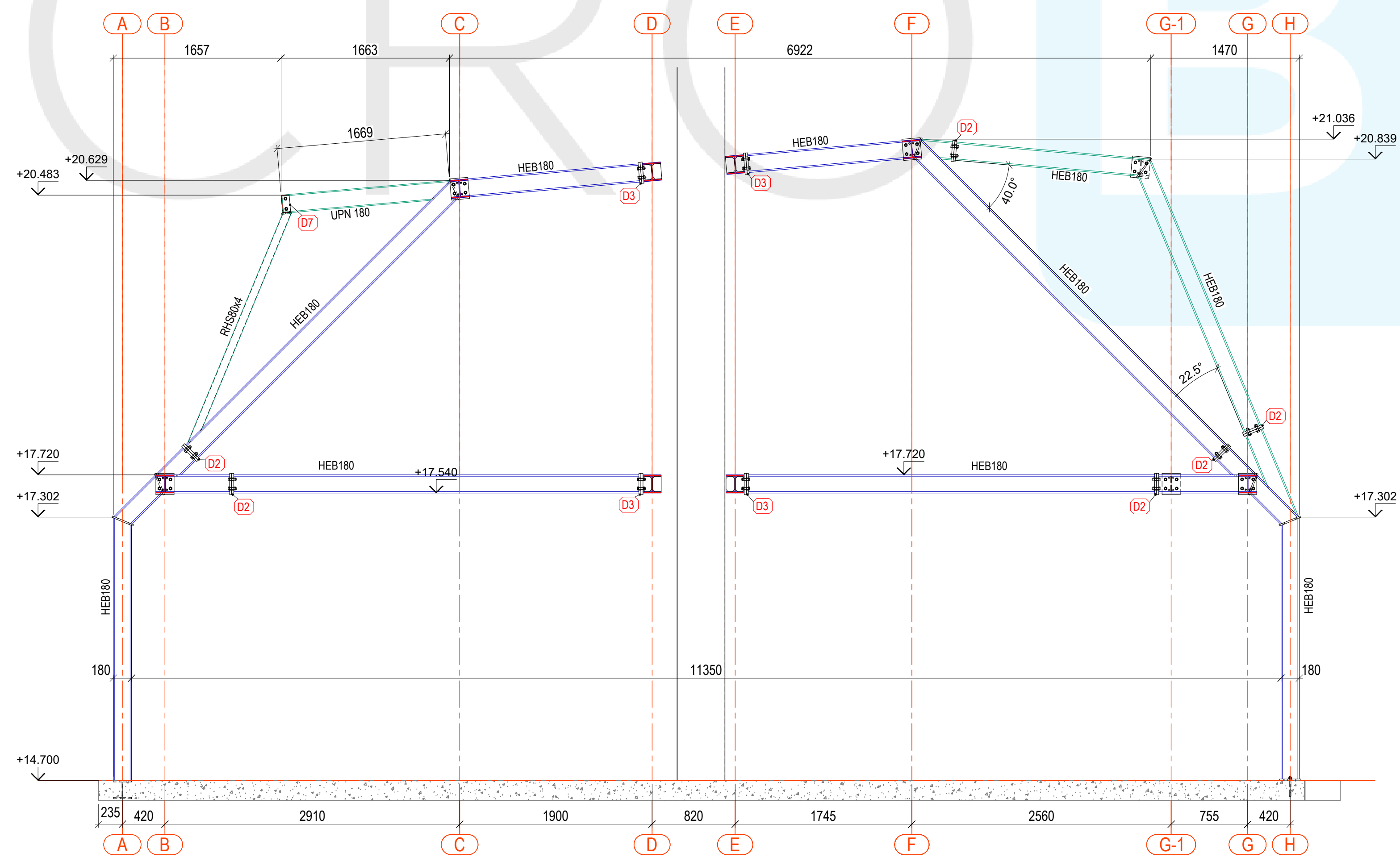
GRID LINE 8 + 18 Scale: 1:33 1/3
