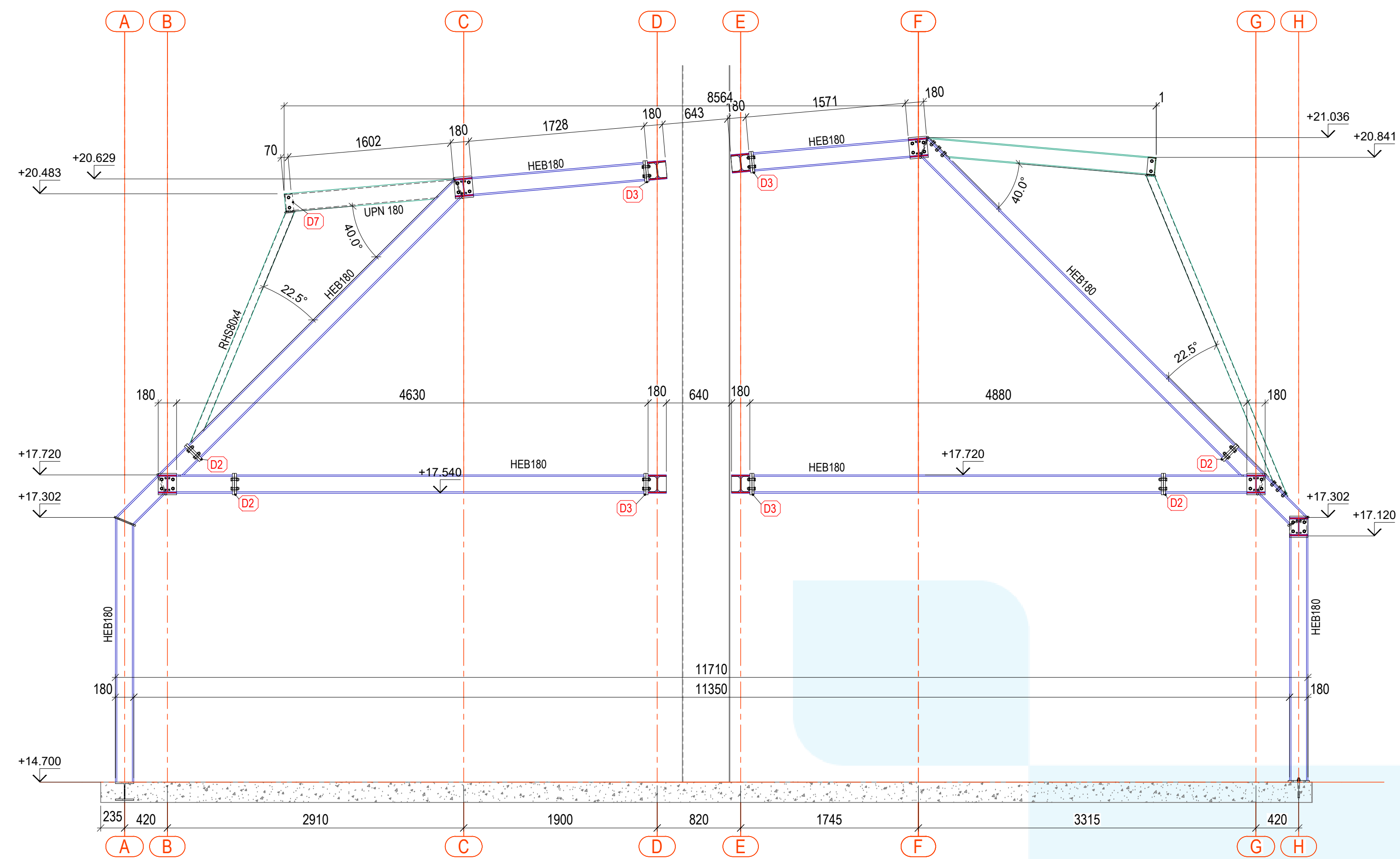
GRID LINE 9 + 19 Scale: 1:33 1/3
