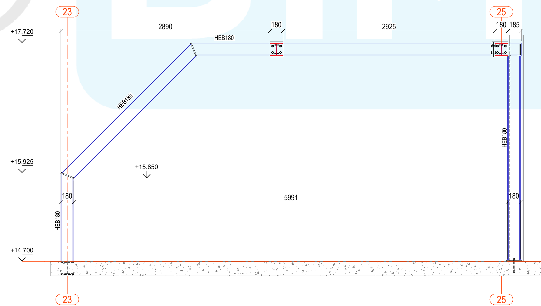
GRID LINE S Scale: 1:25
